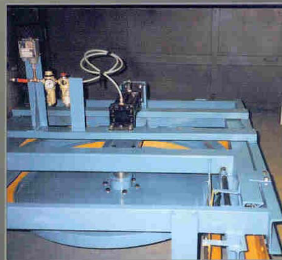
Air operated chain take up
